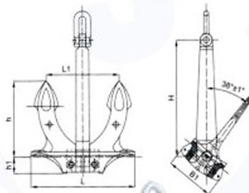
Type B Hall Anchor
